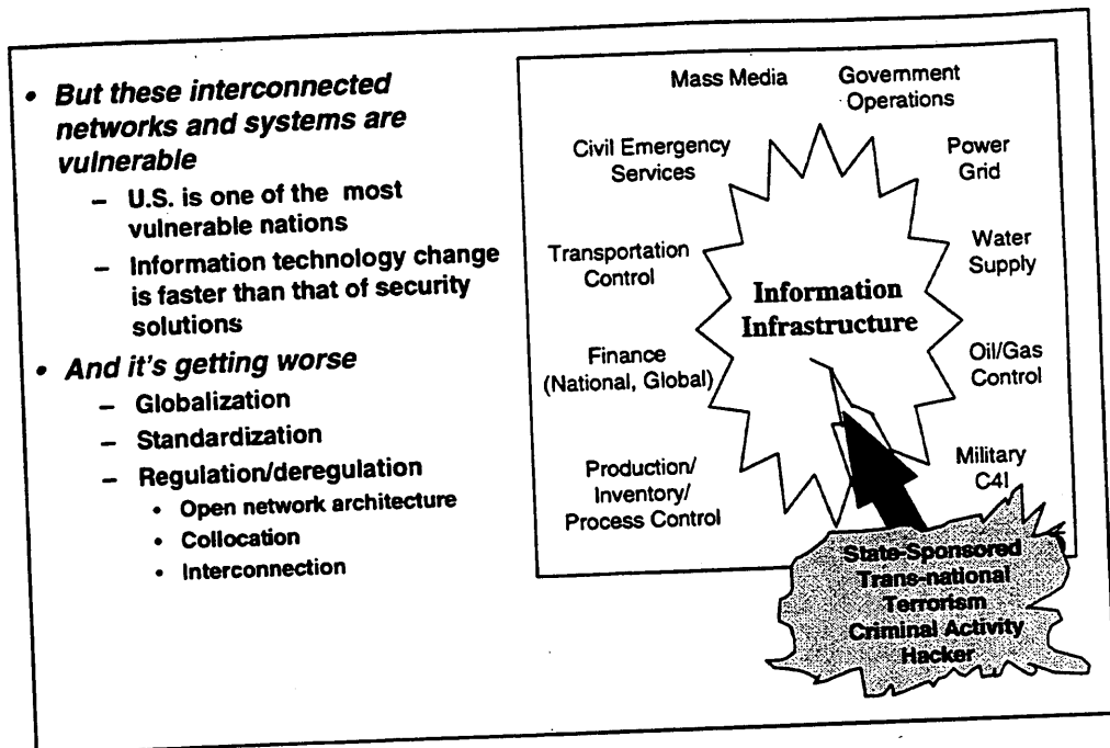
Exhibit 2-3. Vulnerabilities
